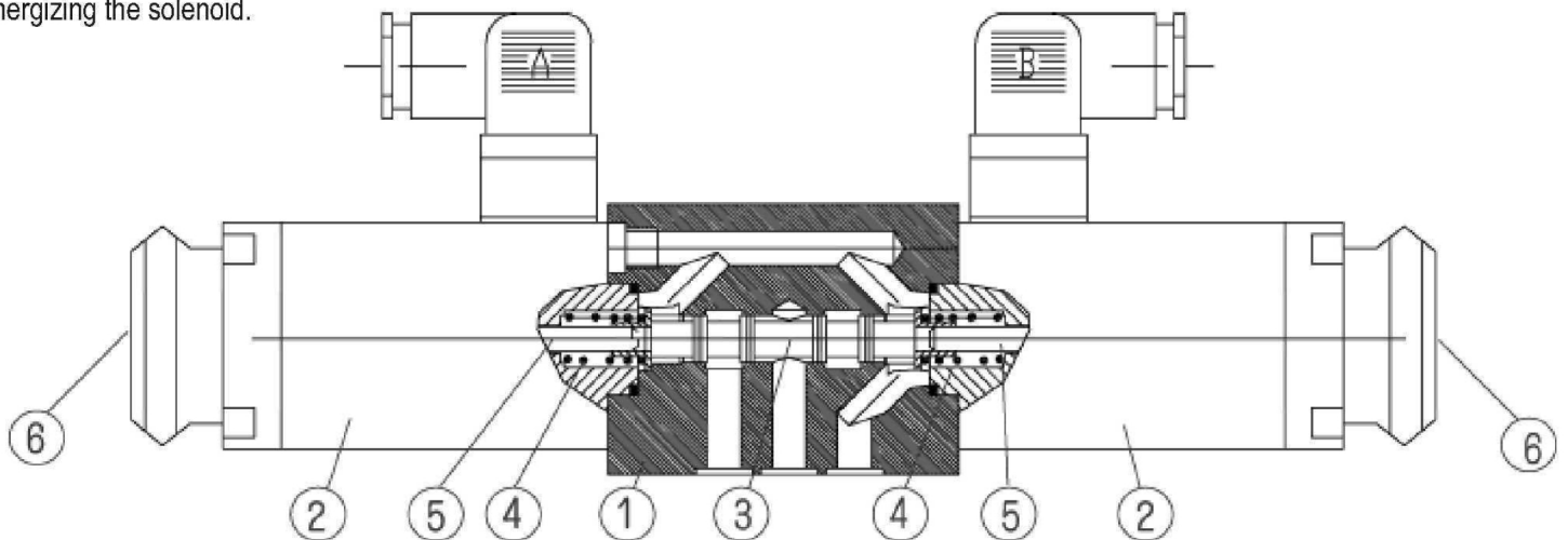
Type WE5
