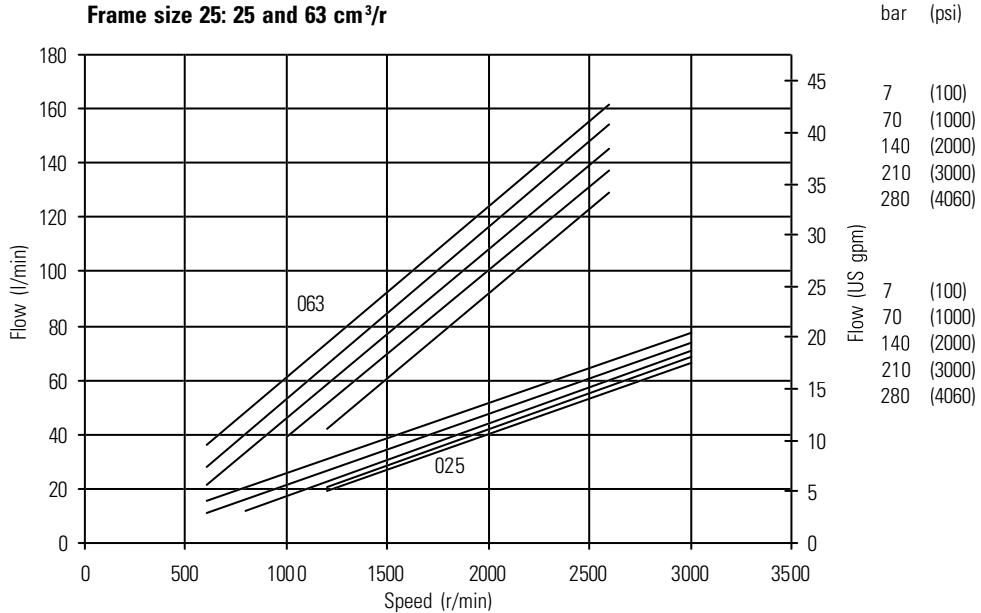
Frame size 25: 25 and 63 cm 3 /r
