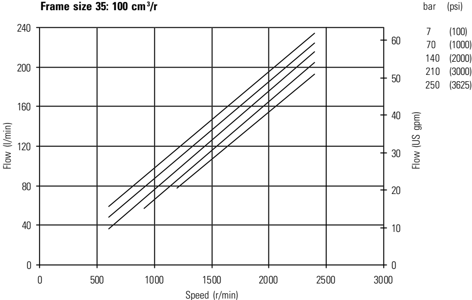
Frame size 35: 100 cm 3 /r
