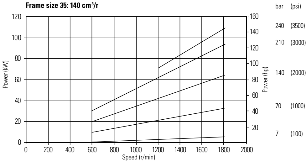
Frame size 35: 140 cm 3 /r
