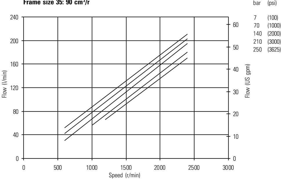
Frame size 35: 90 cm 3 /r
