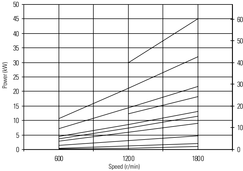
Frame 25: 20 and 50 cm 3 /r
