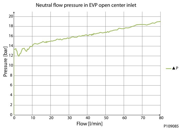
Neutral by-pass pressure drop characteristic (open center)
