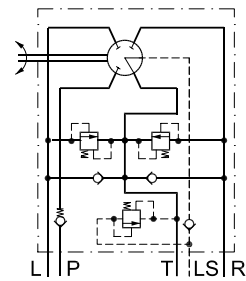
OSPC LS: Steering unit load sensing with integrated valve functions for flange on priority valve OLSA
