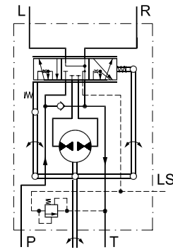
OSPCX LS Load sensing dynamic
