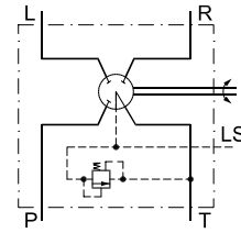
OSPL LS (OLS) Load sensing dynamic
