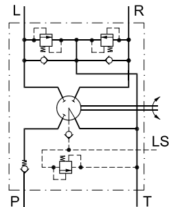
OSPC LS: Steering unit load sensing with integrated valve functions for in line priority valve OLS
