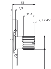
Shaft Code 4
