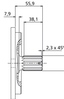
Shaft Code 3
