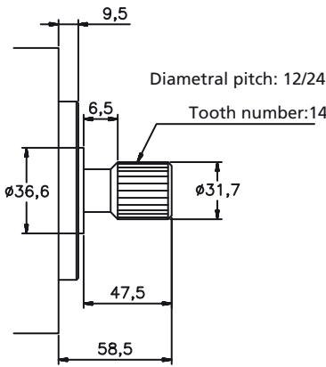
N°11 Shaft
