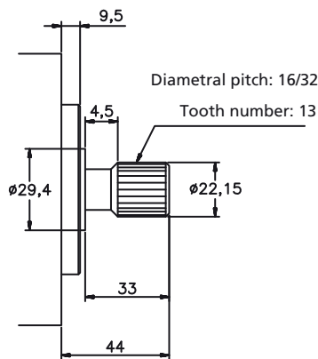
N°11 Shaft
