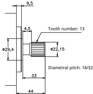
N°11 Shaft
