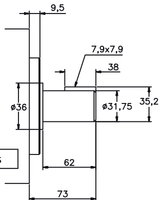
N°1 Shaft
