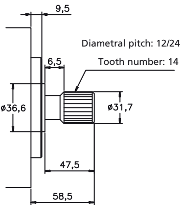
N°11 Shaft
