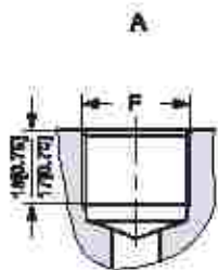
A: G Main port E: ISO 228/1 – G 3/4
