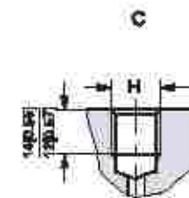
C: G Drain/release port H: ISO 228/1 – G 1/4
