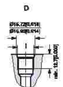
D: UNF Drain port I: 7/8 – 18 UNF O-ring boss port
