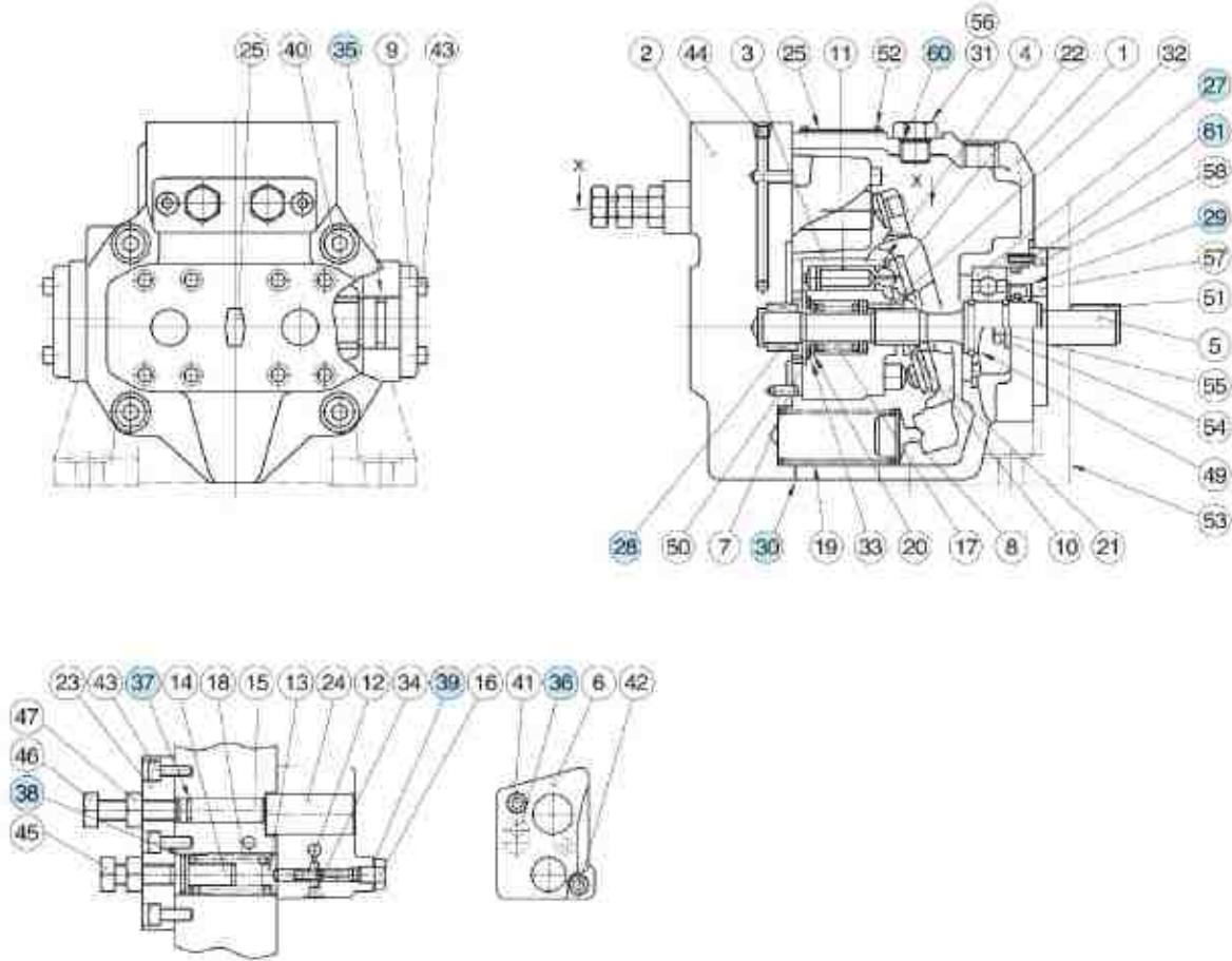
Section X-X
