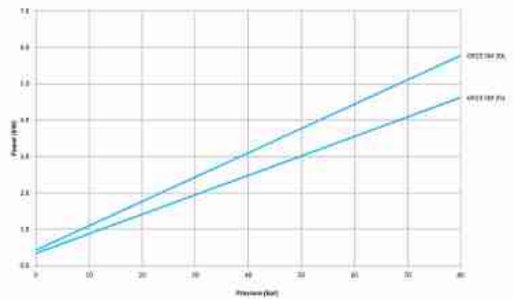
Power GR25 5M @ 2750 RPM - 68 cSt
