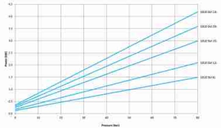
Power GR20 5M @ 2750 RPM - 68 cSt
