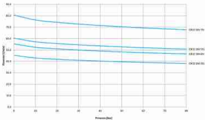
Flowrate GR32 5M @ 2750 RPM - 68 cSt
