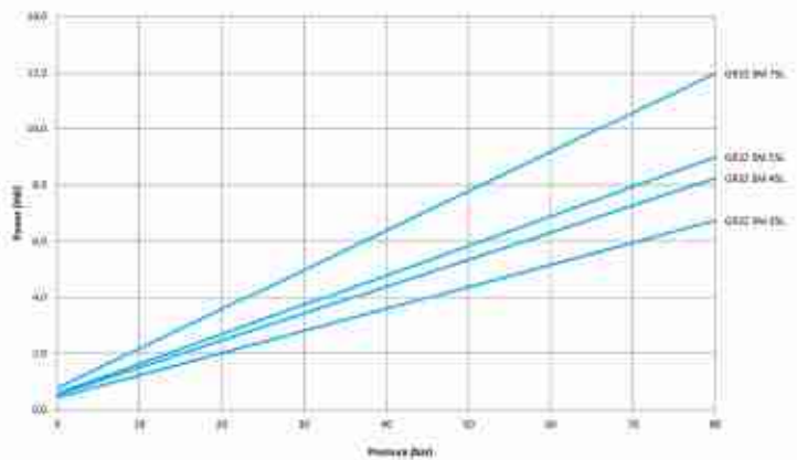
Power GR32 5M @ 2750 RPM - 68 cSt
