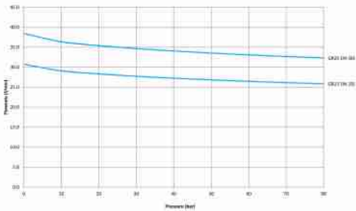
Flowrate GR25 5M @ 2750 RPM - 68 cSt
