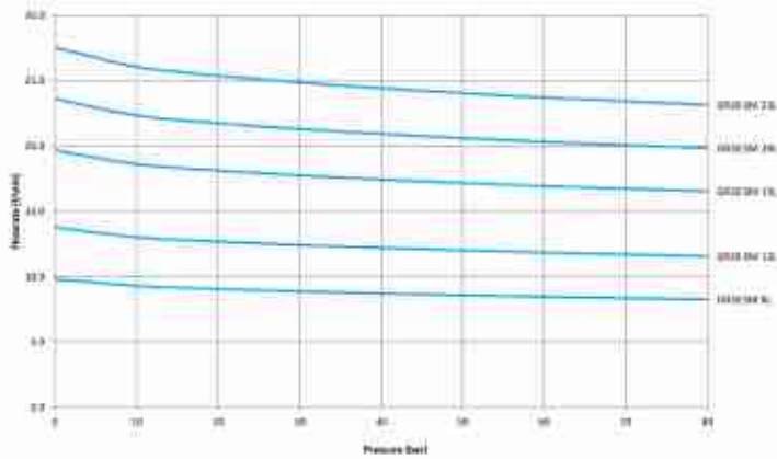
Flowrate GR20 5M @ 2750 RPM - 68 cSt
