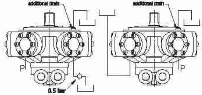
Axis vertical, shaft up
