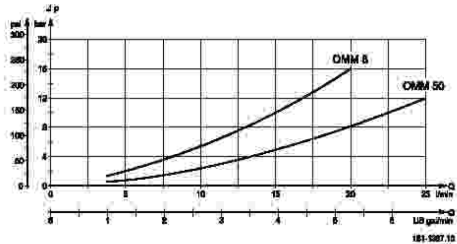
The curve applies to an unloaded motor shaft and an oil viscosity of 35 mm 2 /s [165 SUS]
