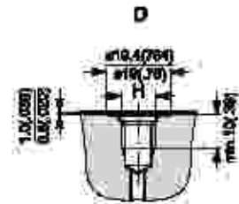
D: UNF drain ports H: 1/8 - 24 UNF O-ring port
