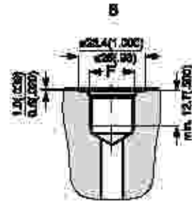
B: UNF main ports F: 1/8 - 18 UNF O-ring boss port
