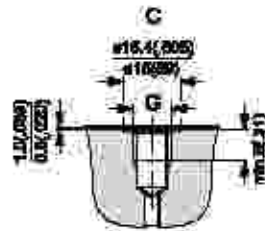
C: G drain ports G: ISO 228/1 - G/a
