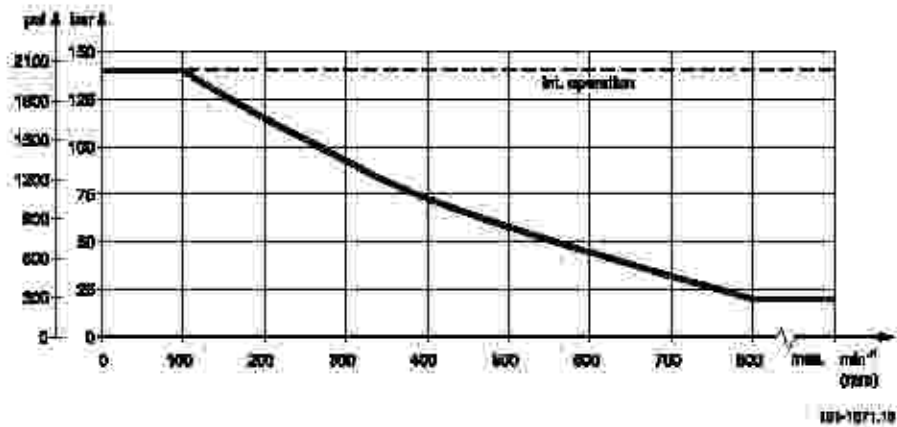
Max. return pressure without drain line or max. pressure in drain line
